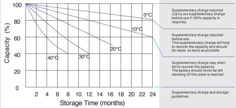
Storage characteristic
